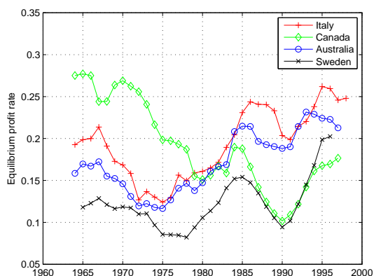
Figure 21: Equilibrium rate \bar{r} .
